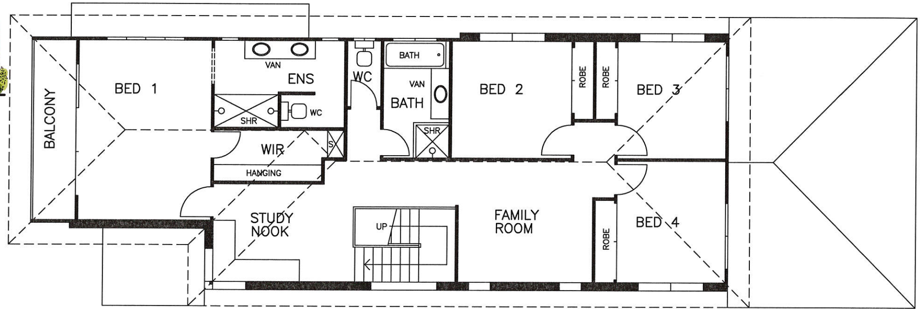
UPPER FLOOR PLAN
